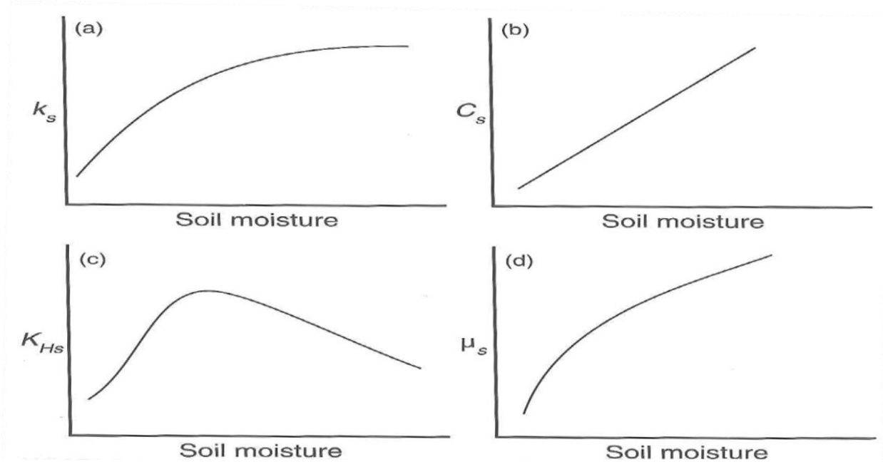
Figure 3. Dependence of (a) thermal conductivity, (b) heat capacity, (c) thermal diffusivity, and (d) thermal admittance on soil moisture. Figure reproduced from Warner (2011), their Figure 5.2.
